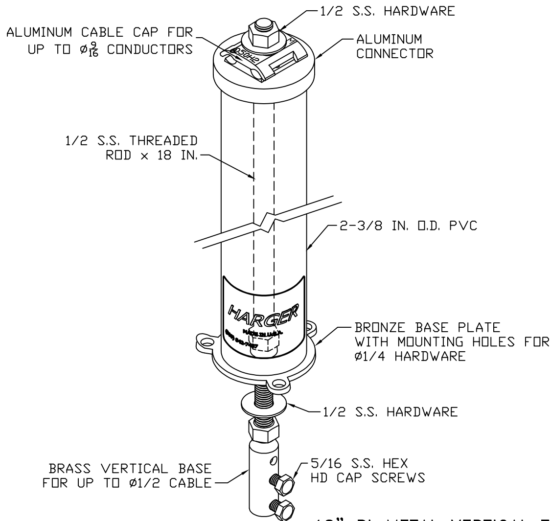
18" BI-METAL VERTICAL THRU ROOF ALUMINUM ROOF CONDUCTOR TO COPPER DOWNLEAD
