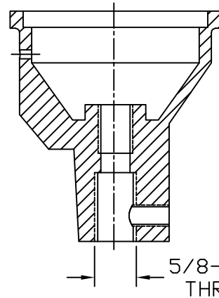
SECTION A-A BRONZE FLOOR GROUND RECEPTACLE
