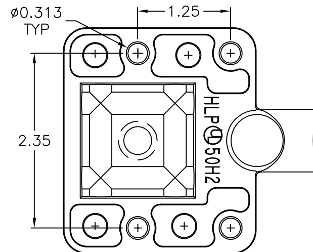
BASE DETAIL
